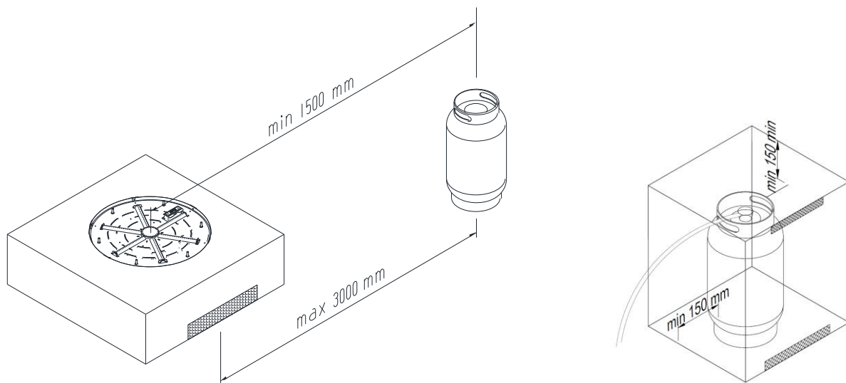
Picture 3 – Gas cylinder distance
