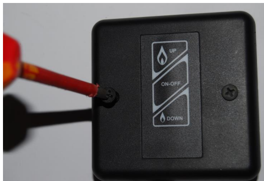
Photo 6 – Wallswitch front panel installation
