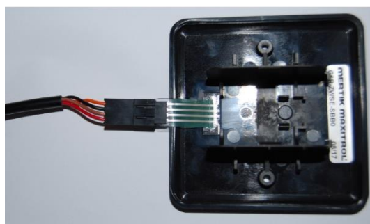
Photo 12 – Wall Switch connection and serial number location
